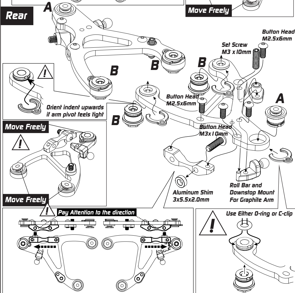
Roll Bar and Downstop Mount For Graphite Arm XP-11190
